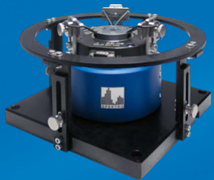
SE-09 Calibration Vibration Exciter for High Frequencies
